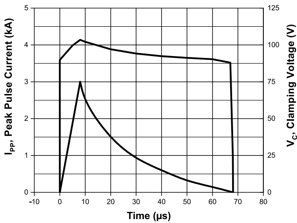
8x20µs Surge Response: CAK3-076C
