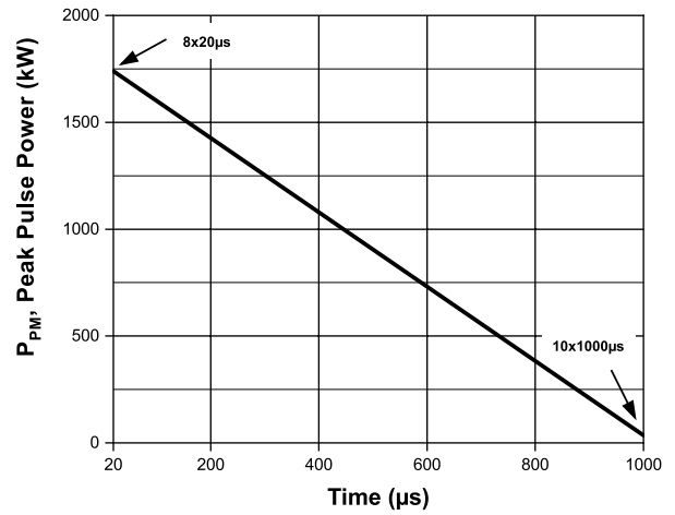
Peak Pulse Power: CAK6-190C
