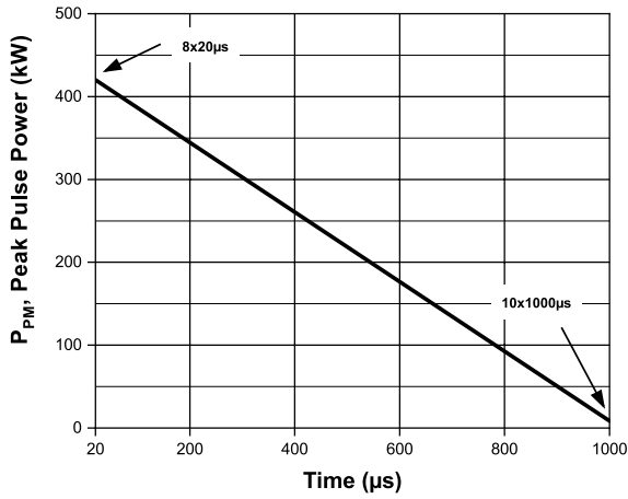
Peak Pulse Power: CAK3-076C
