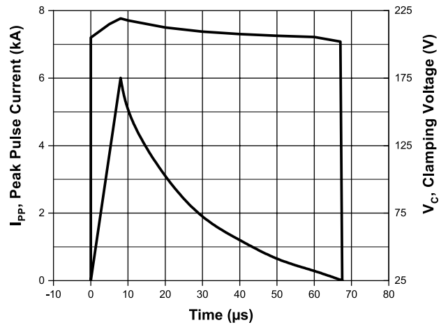
8x20µs Surge Response: CAK6-190C
