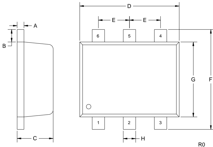
Figure 1: SOT-563 Mechanical Outline
